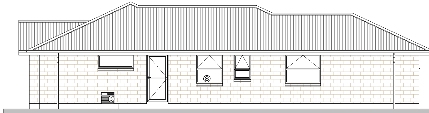
South Elevation
