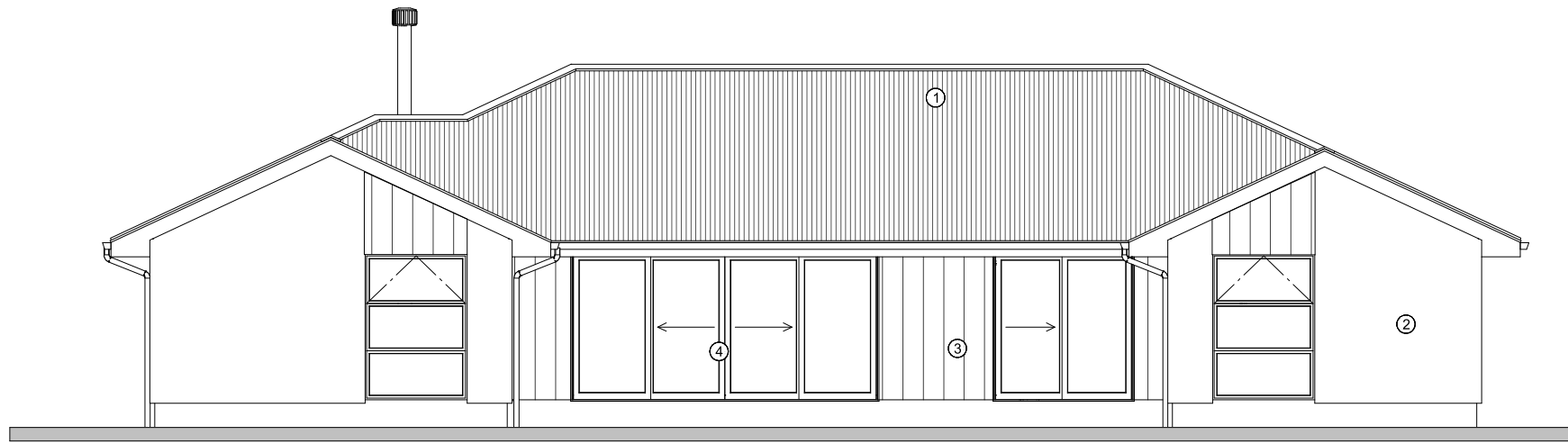
North Elevation
