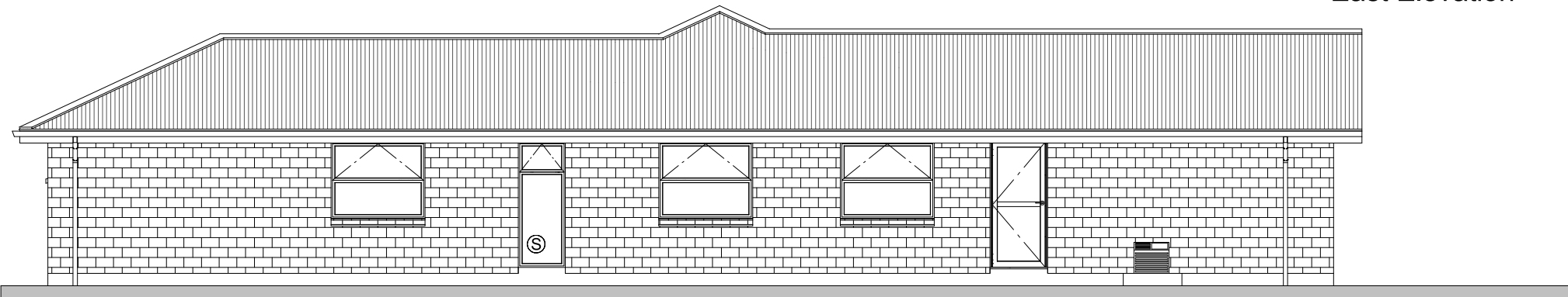
South Elevation
