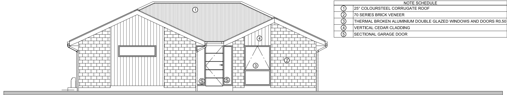
East Elevation
