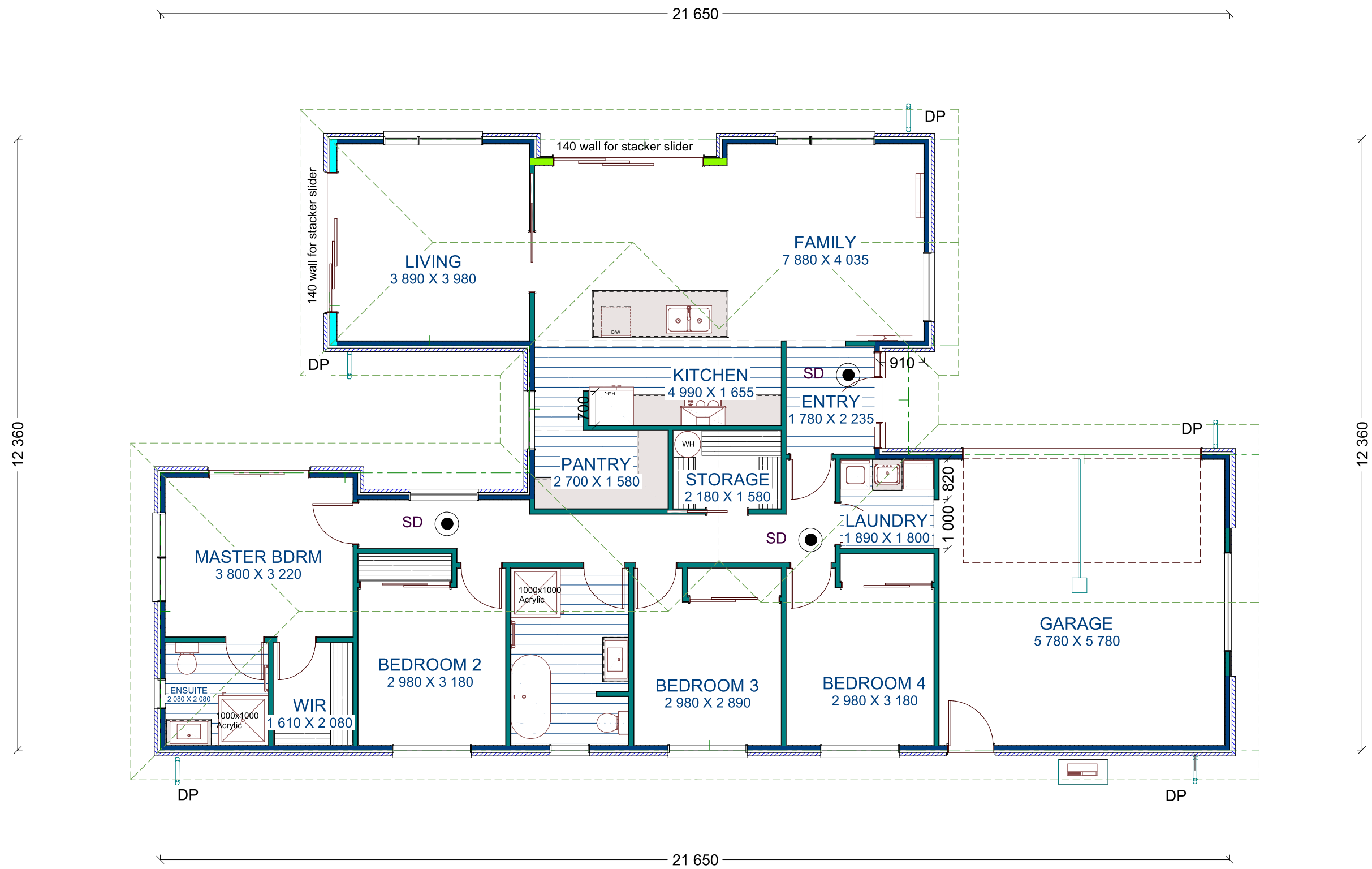
Floor Plan Area 189.9m 2 O/Frame Area 199m 2 O/Found Scale 1-100
