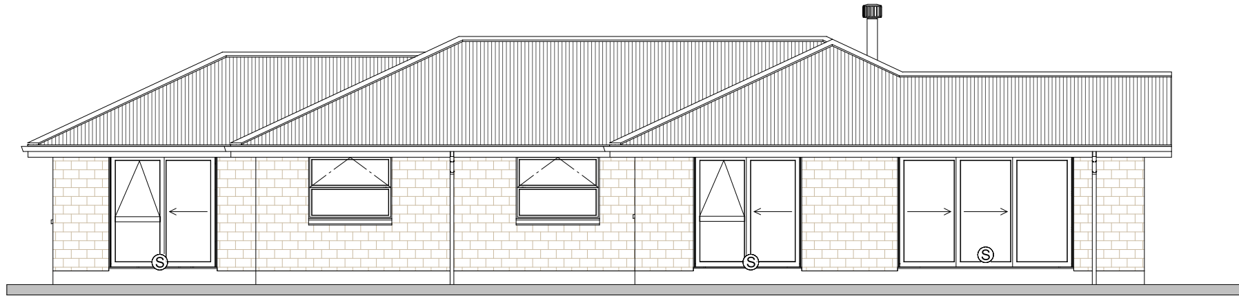
North Elevation
