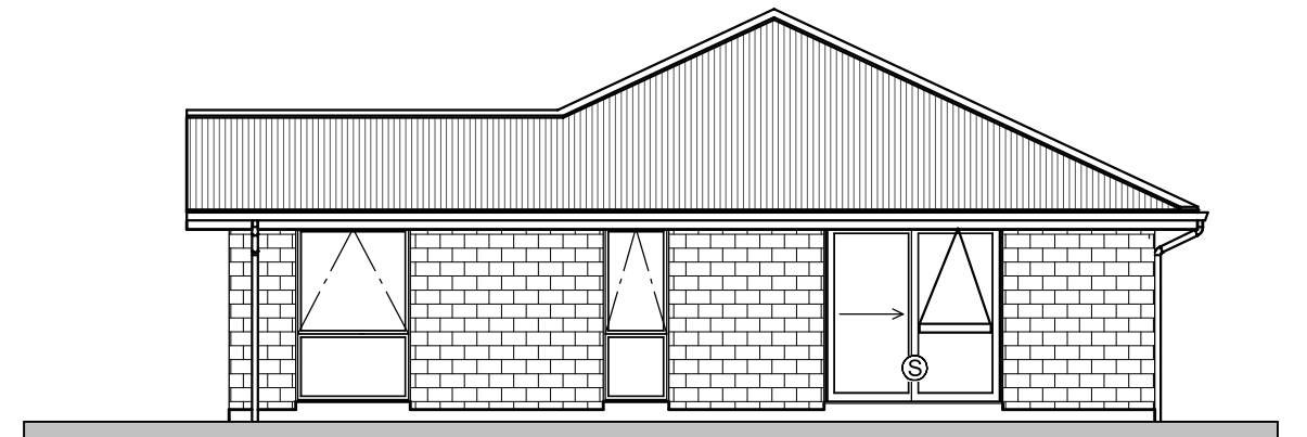
West Elevation
