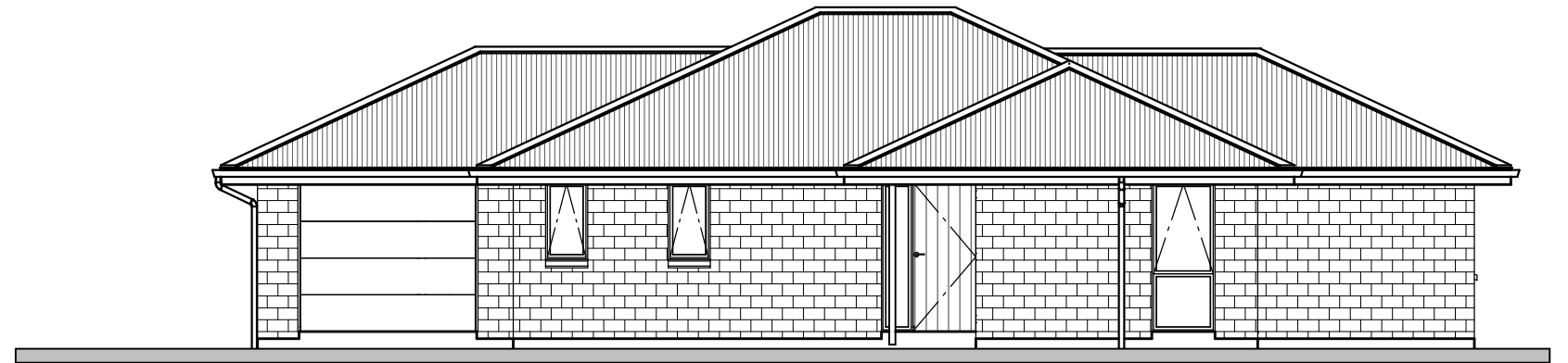
East Elevation
